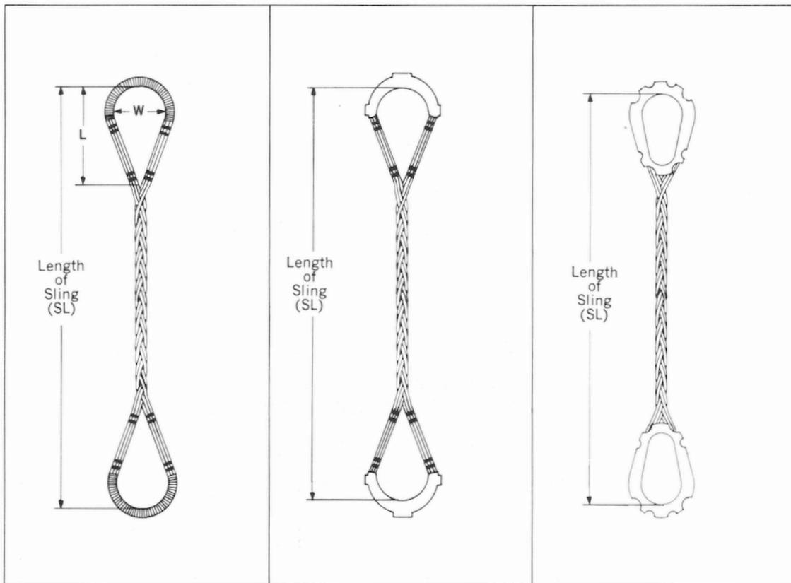
No. 169-B (with slip-thru thimbles)
