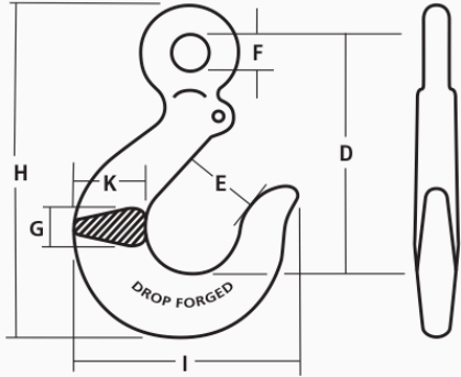
Accoloy® Eye Type Sling Hooks
