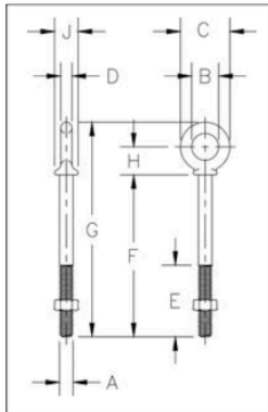
G-277 Shoulder Nut Eye Bolts
