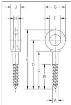
G-275 Screw Eye Bolts
