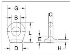
S-264 Pad Eyes
