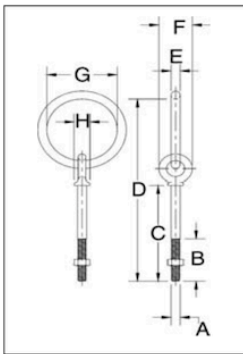
G-257 Shoulder Nut Ring Bolts
